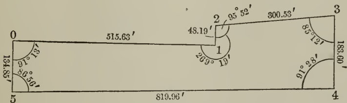
SKETCH OF SURVEY
