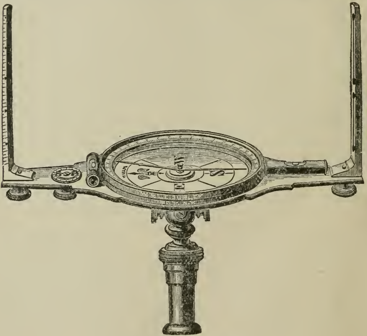
PLAIN SURVEYOR'S COMPASS
