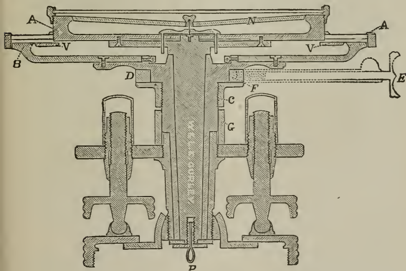
CROSS-SECTION OF THE TRANSIT HEAD
