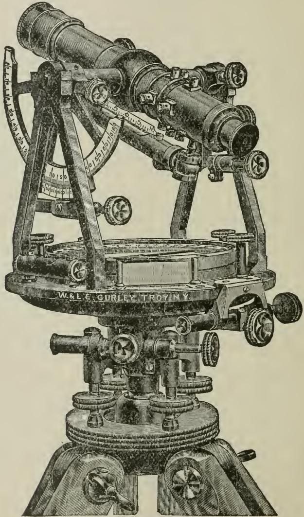
THE TRANSIT
