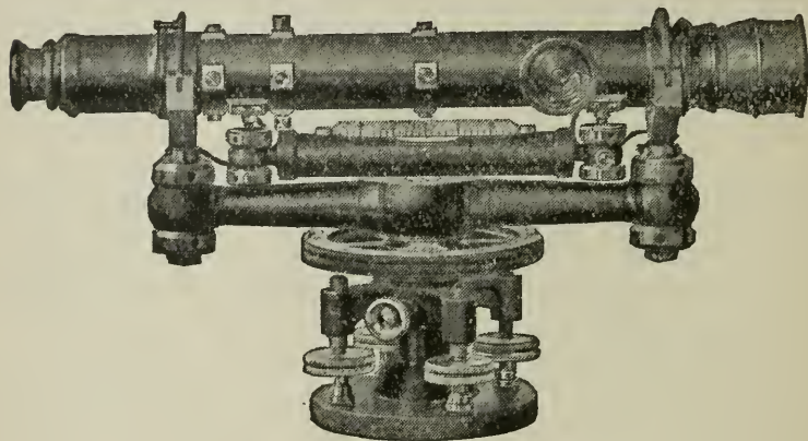
THE LEVEL
