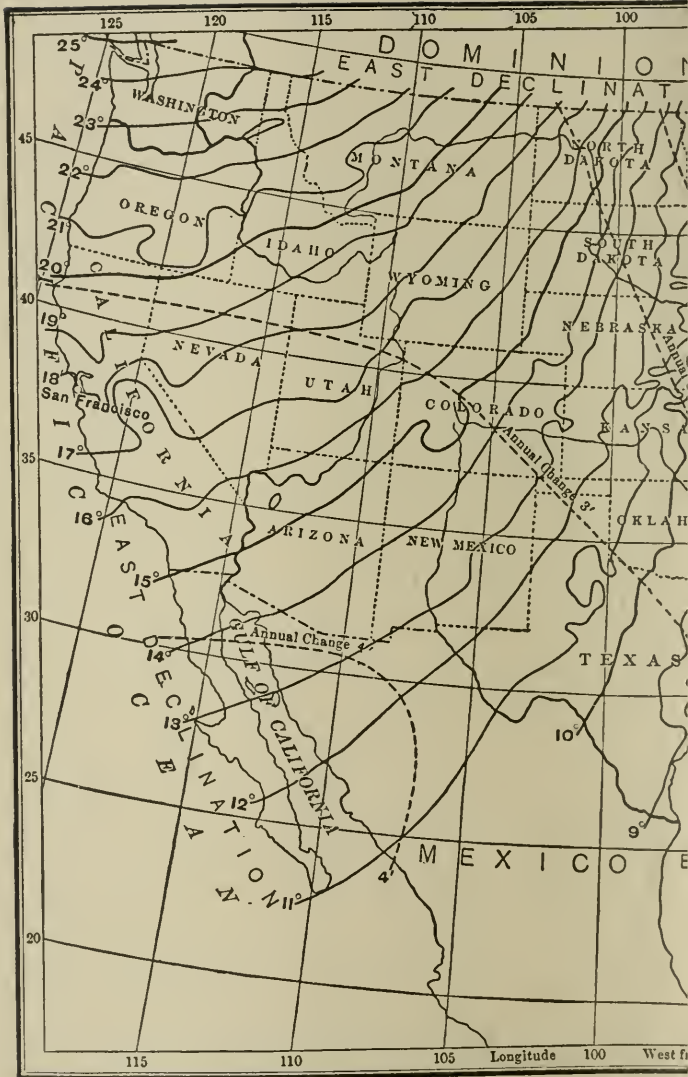
LINES OF EQUAL MAGNETIC DECLINATION AND OF EQUAL ANNUAL MAGNETIC CHANGE IN THE United States Coast
